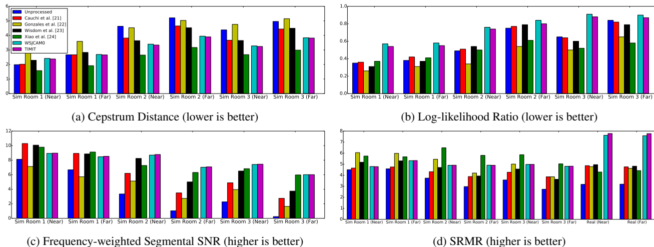
Fig. 1. The speech enhancement results from the REVERB Challenge evaluation data under different test conditions (Sim: simulated data. Real: real recording). For each condition, seven results are reported: unprocessed reverberant and noisy speech as baseline, four results from REVERB Challenge submissions, obtained from http://reverb2014.dereverberation.com/result_se.html , and our proposed approach using speech models learned from WSJCAM0 and TIMIT, respectively.
