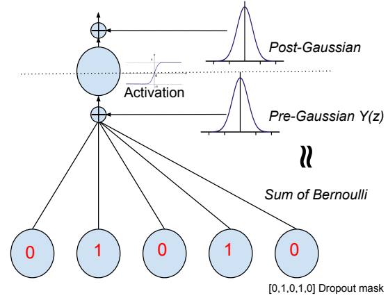
Fig. 1. Illustration of Gaussian stochastic neuron.
