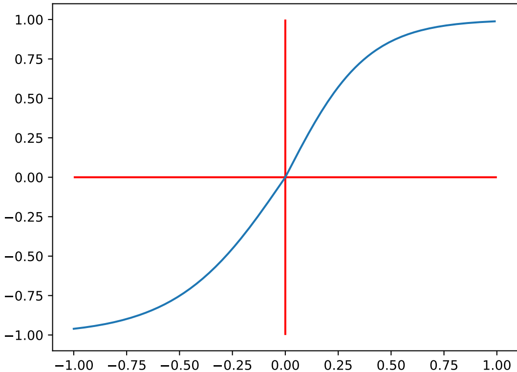
epoch 2-trainRet 61.19
