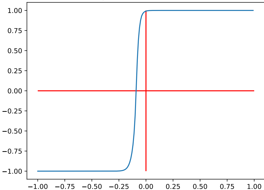
epoch 44-trainRet 21.51
