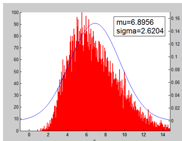
Figure 5 ROS distribution of the main test set.
