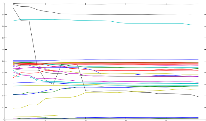
Figure 14 PER on test data for subject 6, with Fbank as features and model trained with the data of this subject. Each curve represents the model trained with the data of a particular channel.
